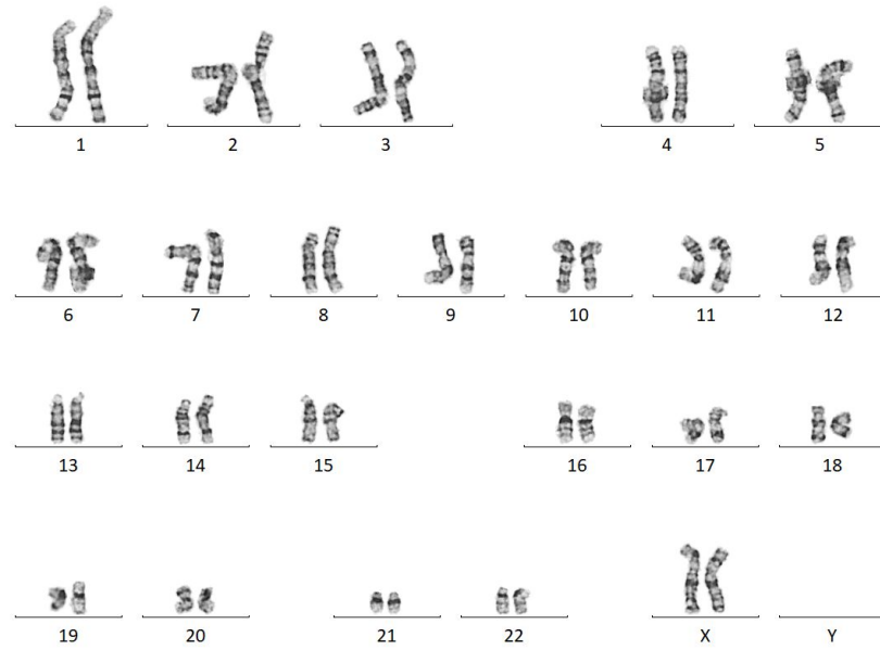
Giemsa-Banding
