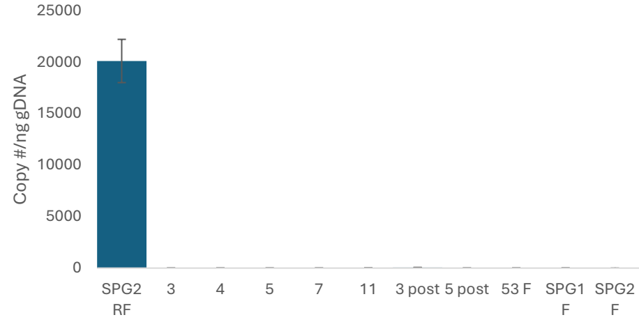
Copy number episomal
