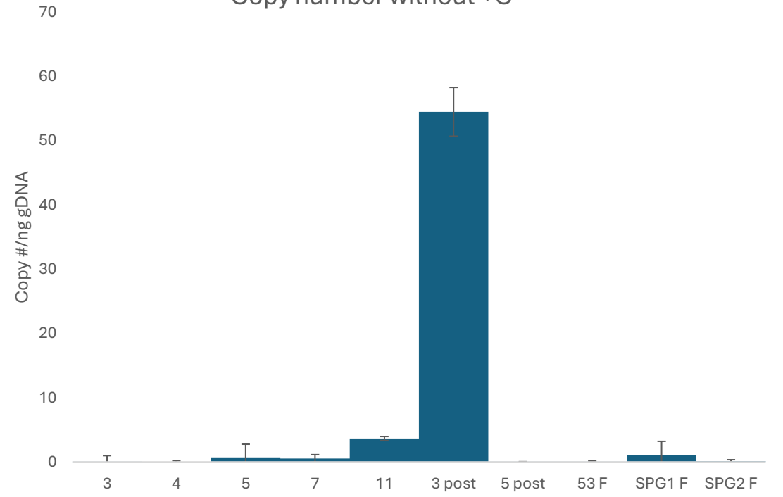
Copy number without +C
