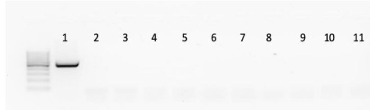
Klf4 (410 pb)
