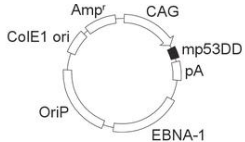
pCE-mp53DD 9.7 kbp
