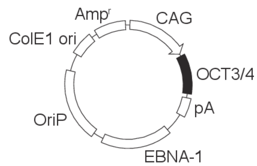
pCE-hOCT3/4 10.5 kbp
