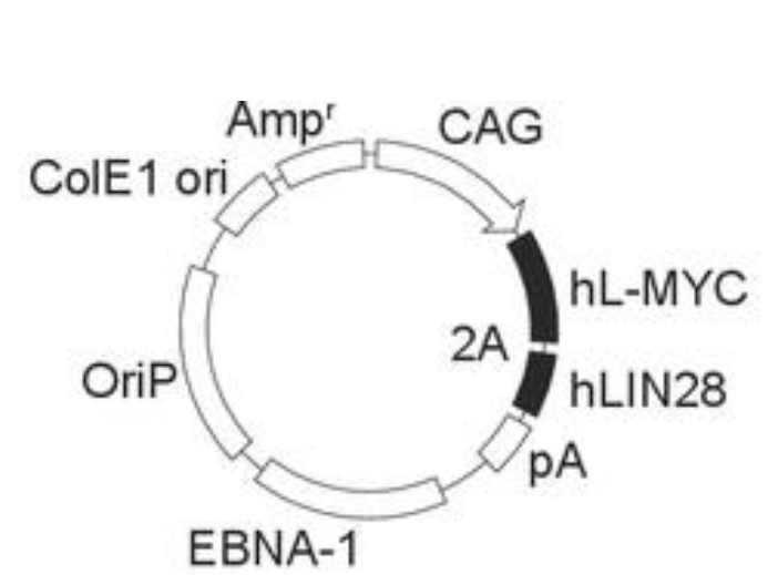
pCE-hUL 11.2 kbp
