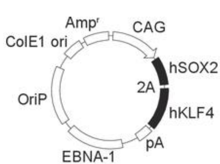
pCE-hSK 11.9 kbp
