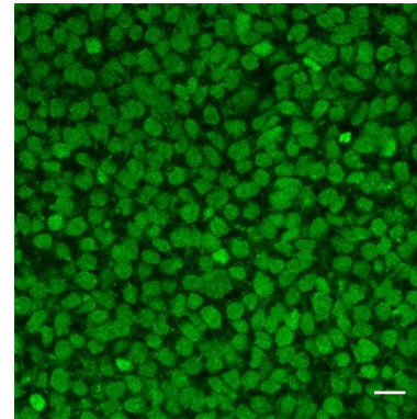
Sox-17
