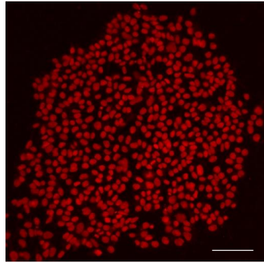
OCT3/4
