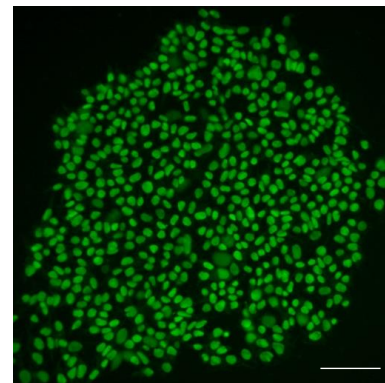
SOX2
