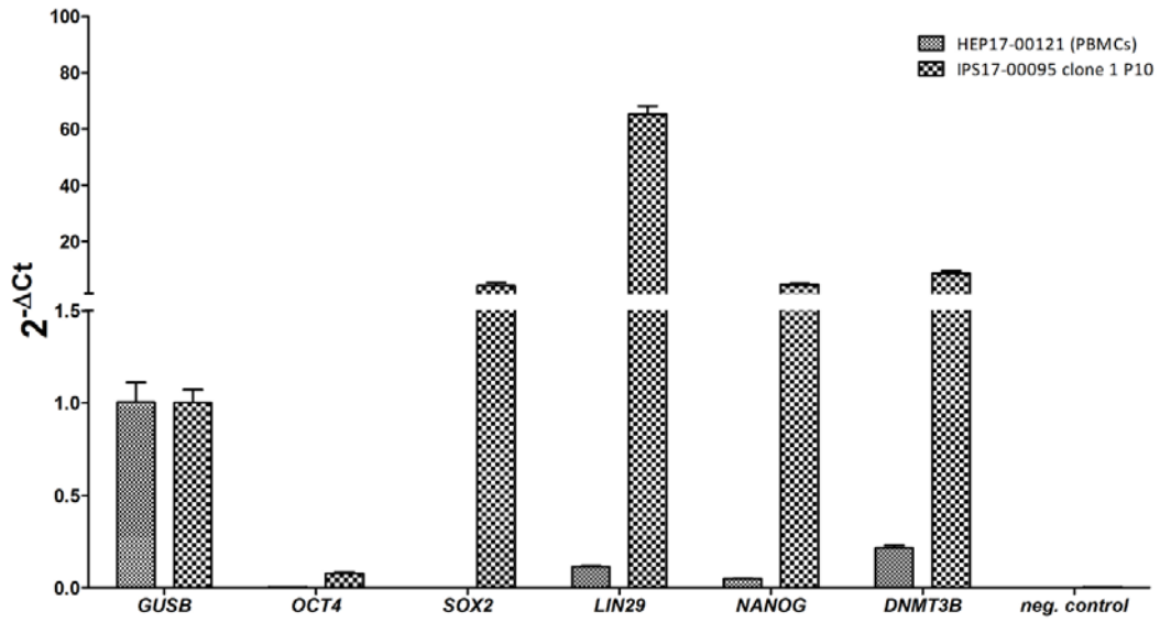
Figure 4: Gene expression of one iPSC clone compared with the parental PBMCs ( \Delta Ct ).
