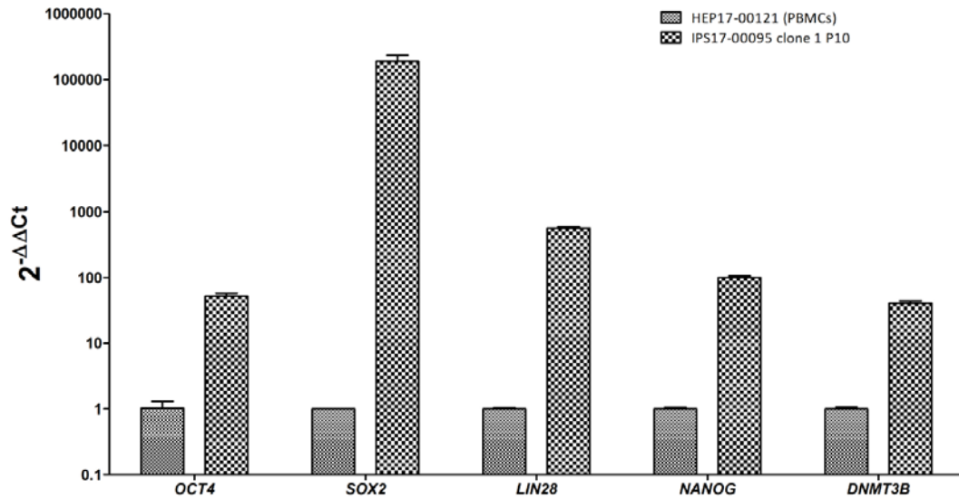
Figure 5: Pluripotency gene upregulation after reprogramming ( \Delta\Delta Ct ). The expression fold difference of the iPSC clone is relative to the parental PBMCs.
