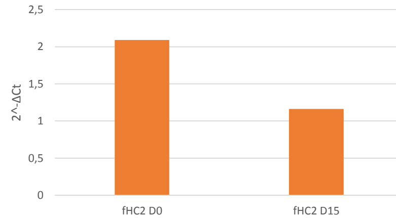
SOX2
