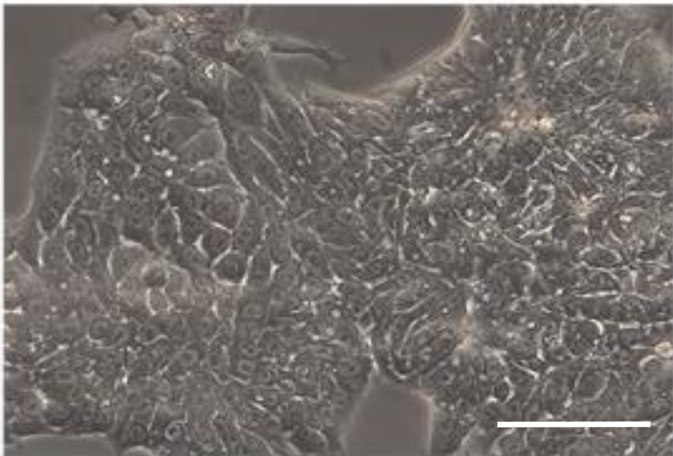
iPS cells morphology. Scale bar: 100 \mu\text{m} .
