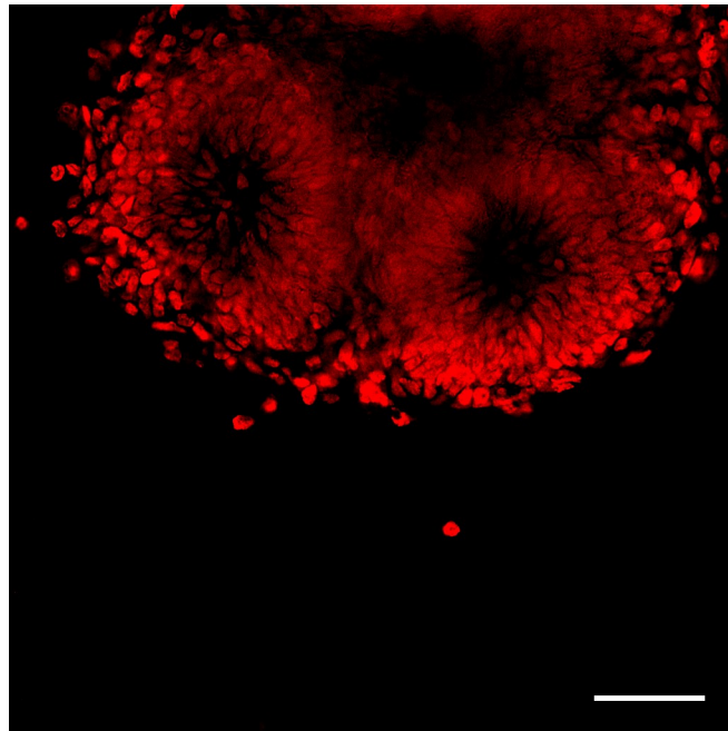
PAX6
