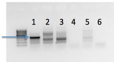
Klf4 (410 pb)
