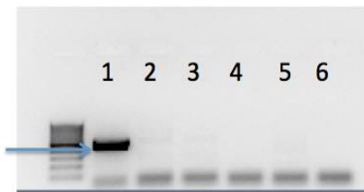
KOS (528 pb)
